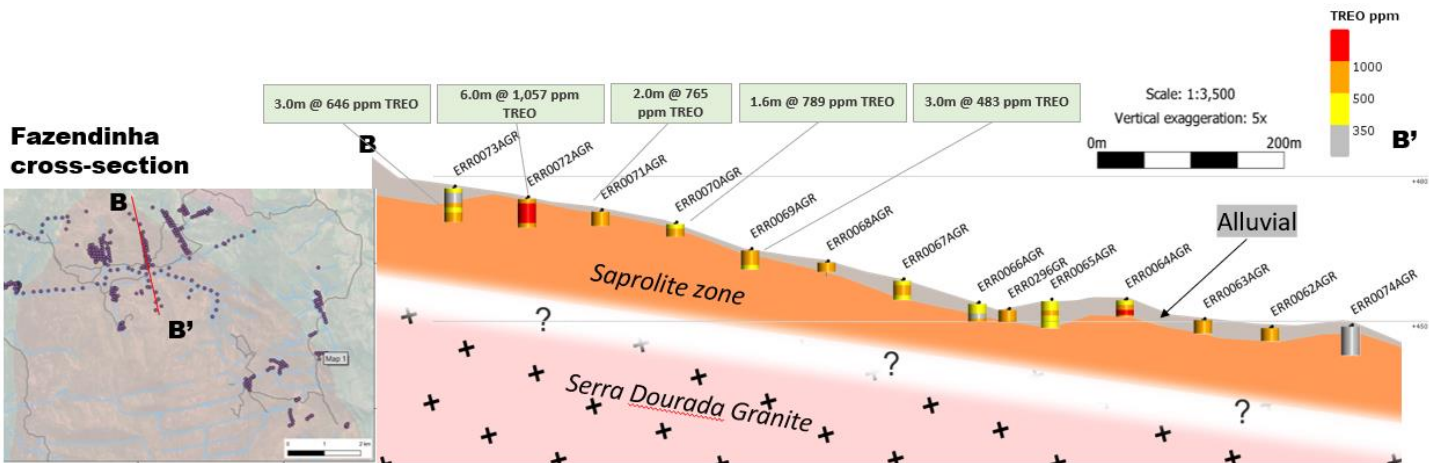
Figure 5: Cross section through Fazendinha prospect at the Bluebush Project. Note the auger drilling rarely penetrates deeply into the saprolite zone.
