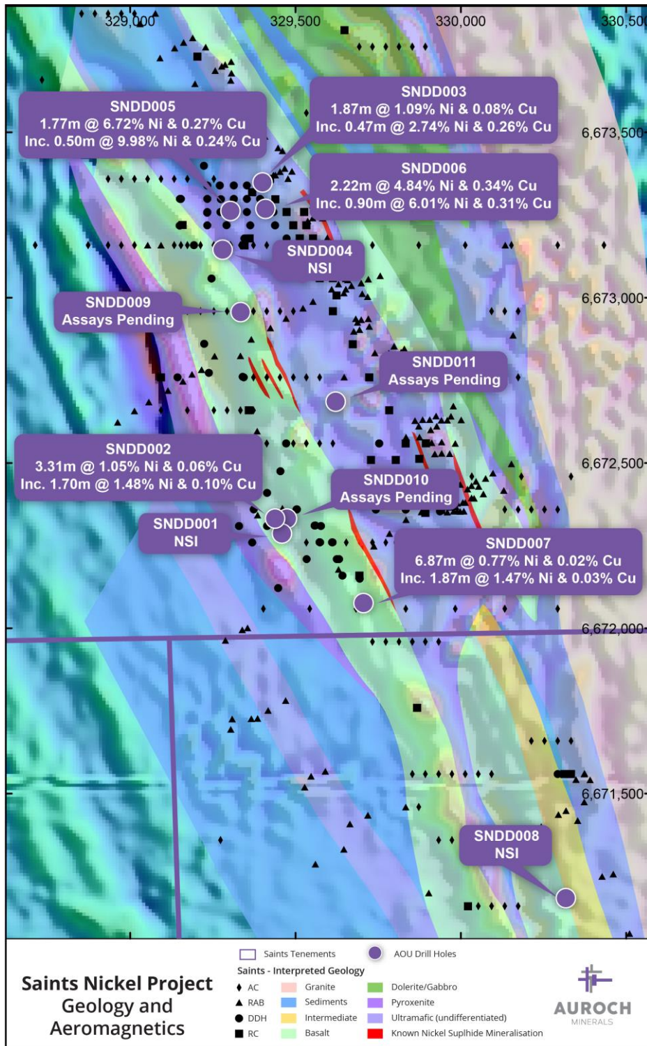
Figure 1 – Plan map of the Saints Nickel Project showing the locations of the eleven drill-holes in relation to geology and aeromagnetics (RTP-1VD)
