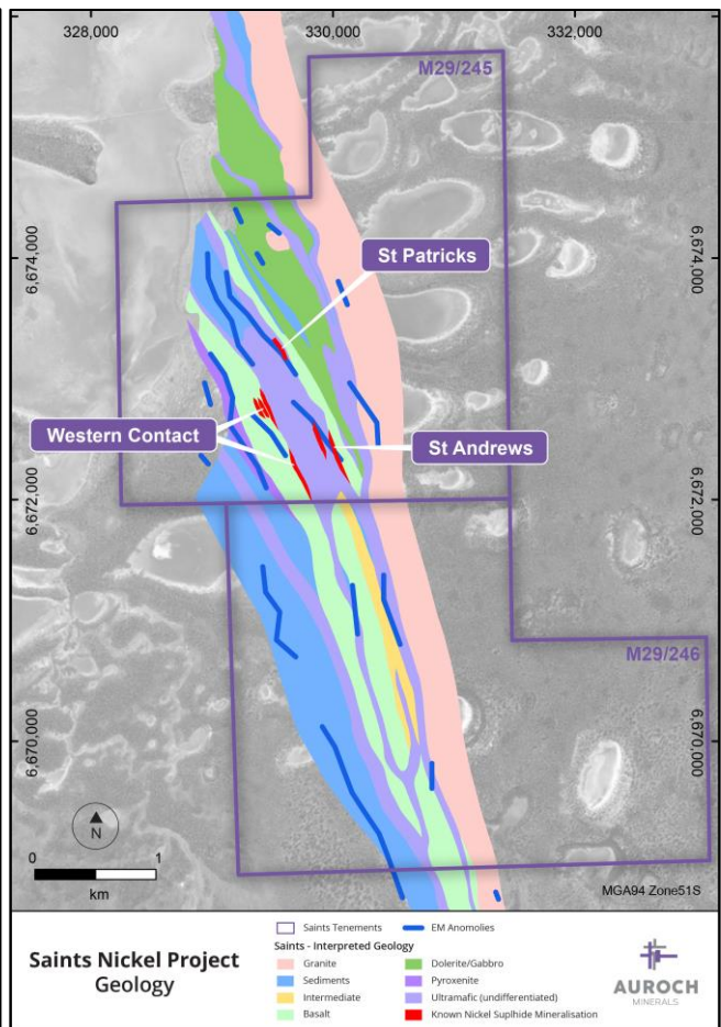
Surface geology map of the Saints Nickel Project highlighting the numerous EM plates (dark blue) in relation to the known nickel sulphide mineralisation (dark red) and ultramafic units (purple).
