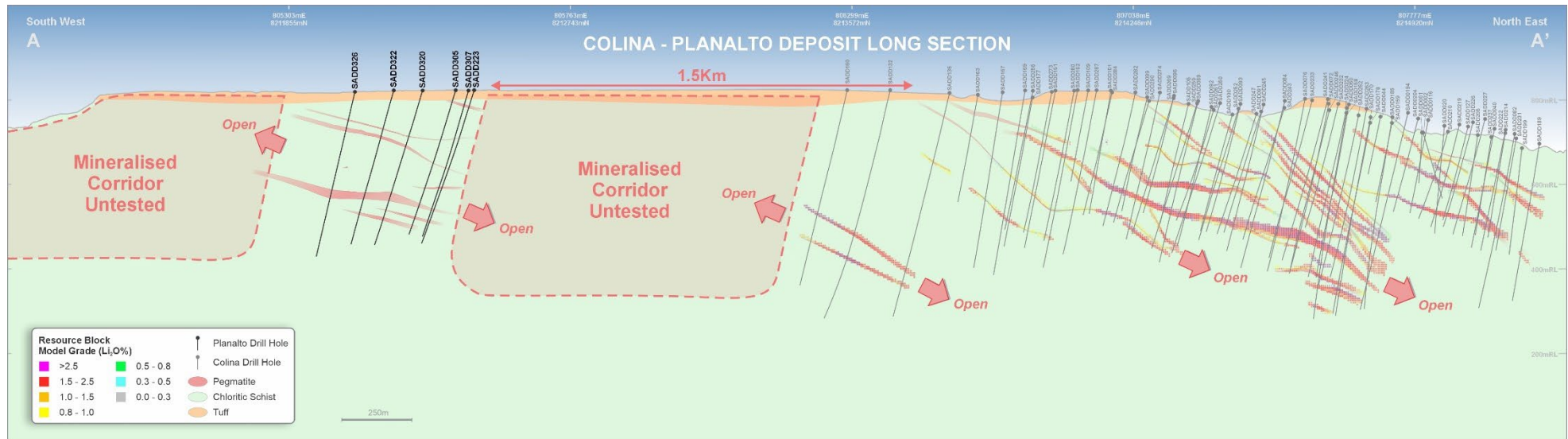
Figure 3: Schematic Longitudinal section the Colina Mineralised system along with the Planalto mineralised system (1.5x exaggeration on the vertical scale).
