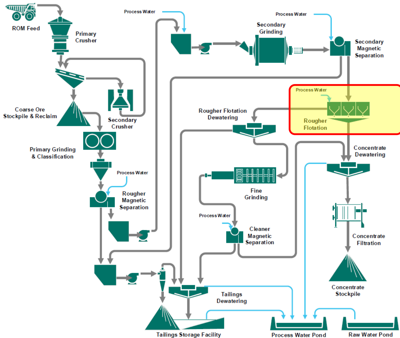
Figure 2 - Razorback Process Flowsheet schematic, highlighting flotation stage
