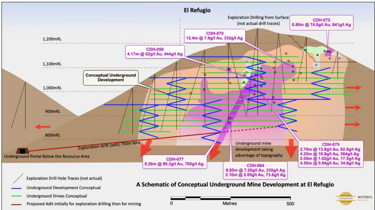
Figure 23: Schematic showing an underground mine access concept for the El Refugio gold-silver deposit, Copalquin District, Mexico.
