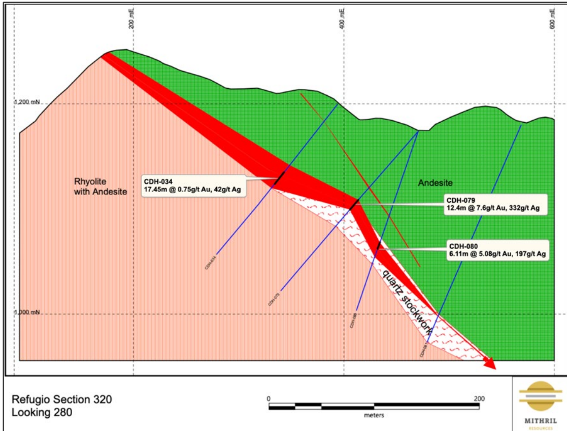
Figure 14: El Refugio cross section 320 showing intercepts for new drill holes CDH-079 & 080, 80 metres east of section 400 shown below in Figure 15
