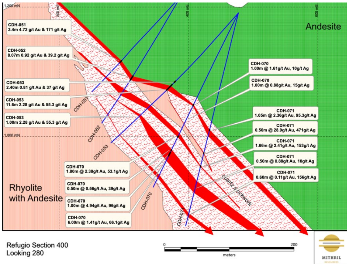
Figure 15: El Refugio cross section 400 showing intercepts at El Refugio 80 metres west of the new intercepts reported in Figure 6.
