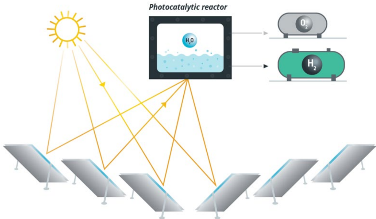
Sparc Green Hydrogen schematic demonstrating combination of concentrated solar and photocatalytic water splitting
