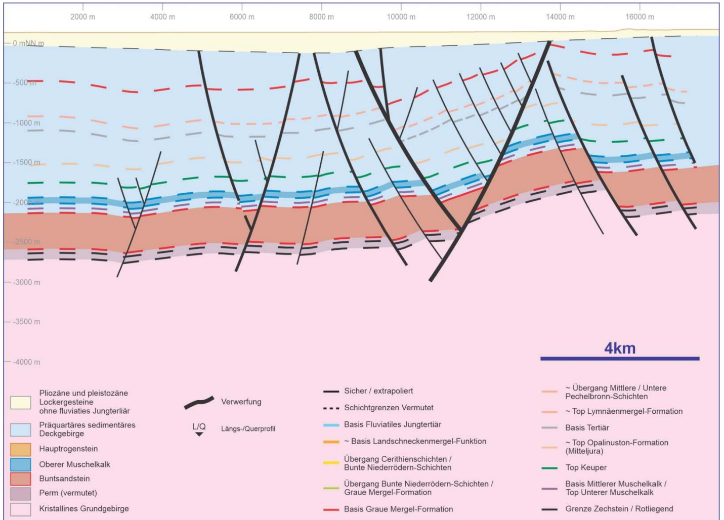
Figure 7: Cross-Section through Mannheim license in Upper Rhine Valley, showing Upper Muschelkalk (dark blue) and Buntsandstein (orange) target sedimentary formations. Cross section location is shown in Figure 1. Publicly available from GeotIS.de
